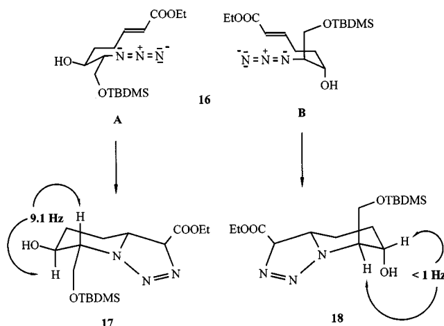
Scheme 5. Stereochemical outcome of the cycloaddition reaction
