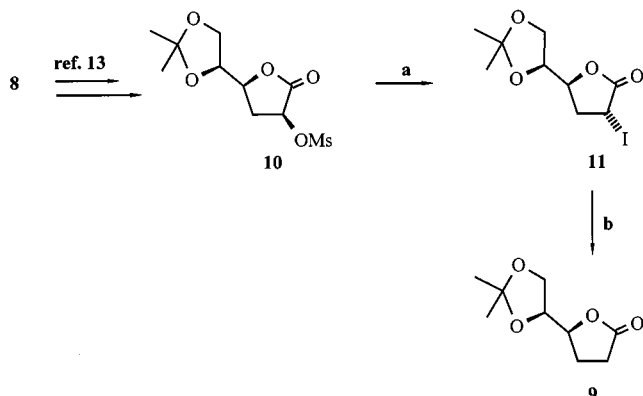
Scheme 2. a) NaI, acetone, reflux, 92%. – b) H 2 , Et 3 N, 10% Pd/C, 20–30 h, 82%.
