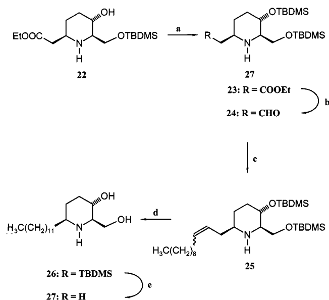
Scheme 7. a) TBDMSCl, imidazole, DMF, 84%; b) \text{DIBALH} , n -pentane, -78^\circ\text{C} , 25 min, 66%; c) \text{Ph}_3\text{P}(\text{CH}_2)_9\text{CH}_3\text{Br} , \text{Na}[\text{Si}(\text{CH}_3)_3]_2 , THF, (i) -40^\circ\text{C} , 60 min, (ii) room temp, 160 min, 79%; d) \text{H}_2 , 10% Pd/C, EtOH, 12 h, 93%; e) \text{HCl} , EtOH, 15 min, then 6 N KOH, 87%
