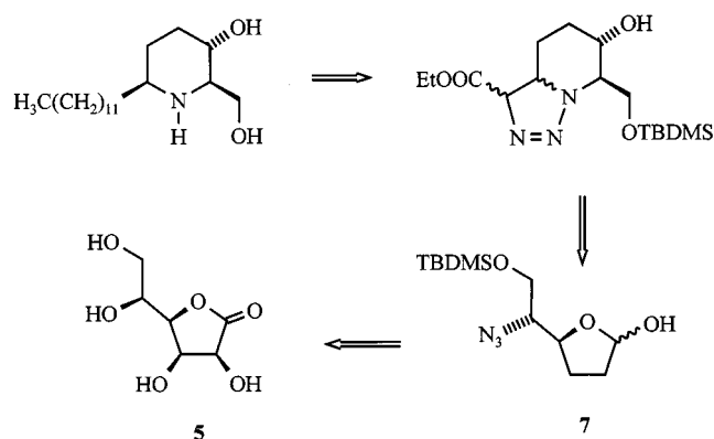
Scheme 1. Retrosynthetic analysis
