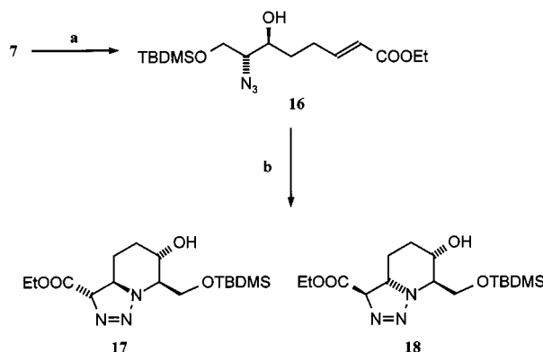
Scheme 4. a) Ph 3 PCHCOOEt, toluene, room temp., 1 d; b) toluene, room temp., 4 d, 98%
